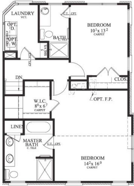
Second Floor 682 SQ. FT.
